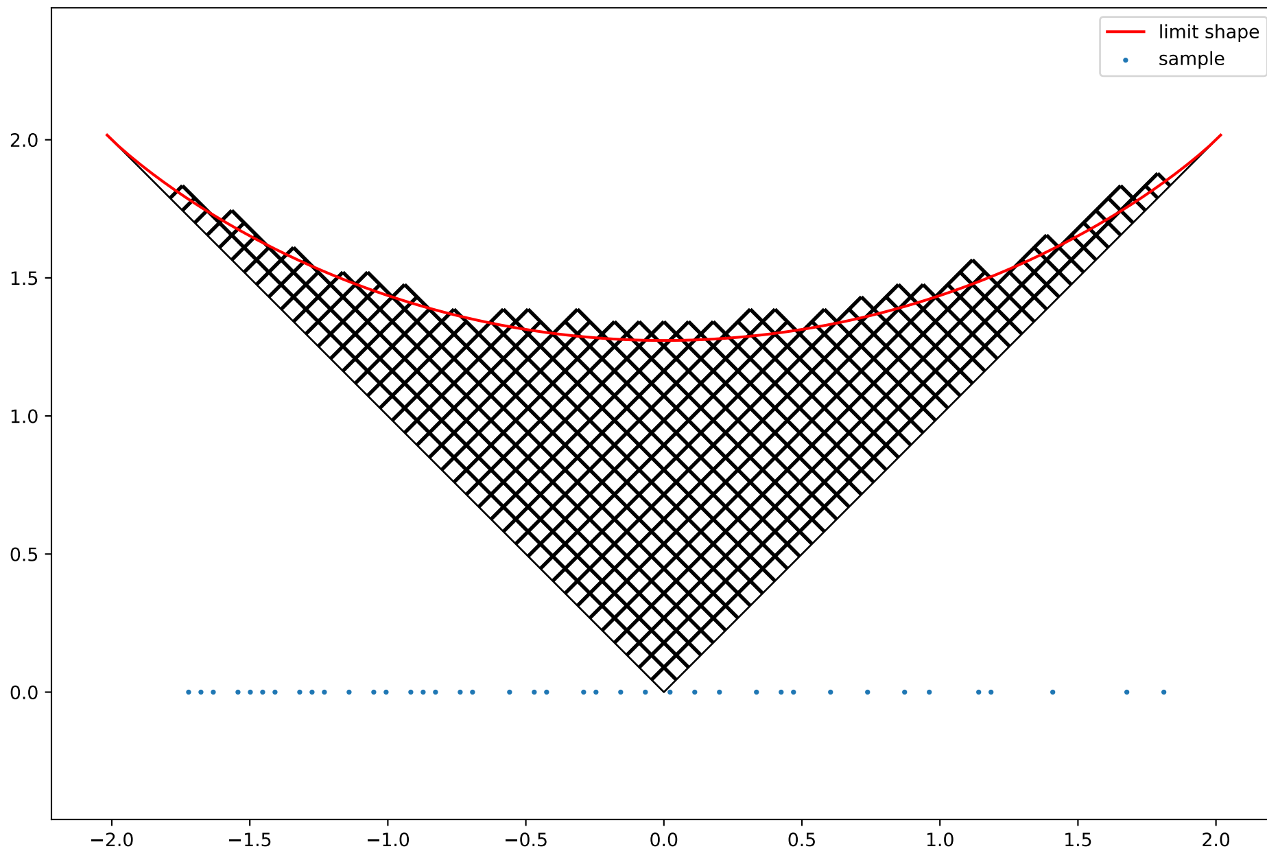
Young diagram associated to Poissonized Plancherel measure with parameter \theta = 500
