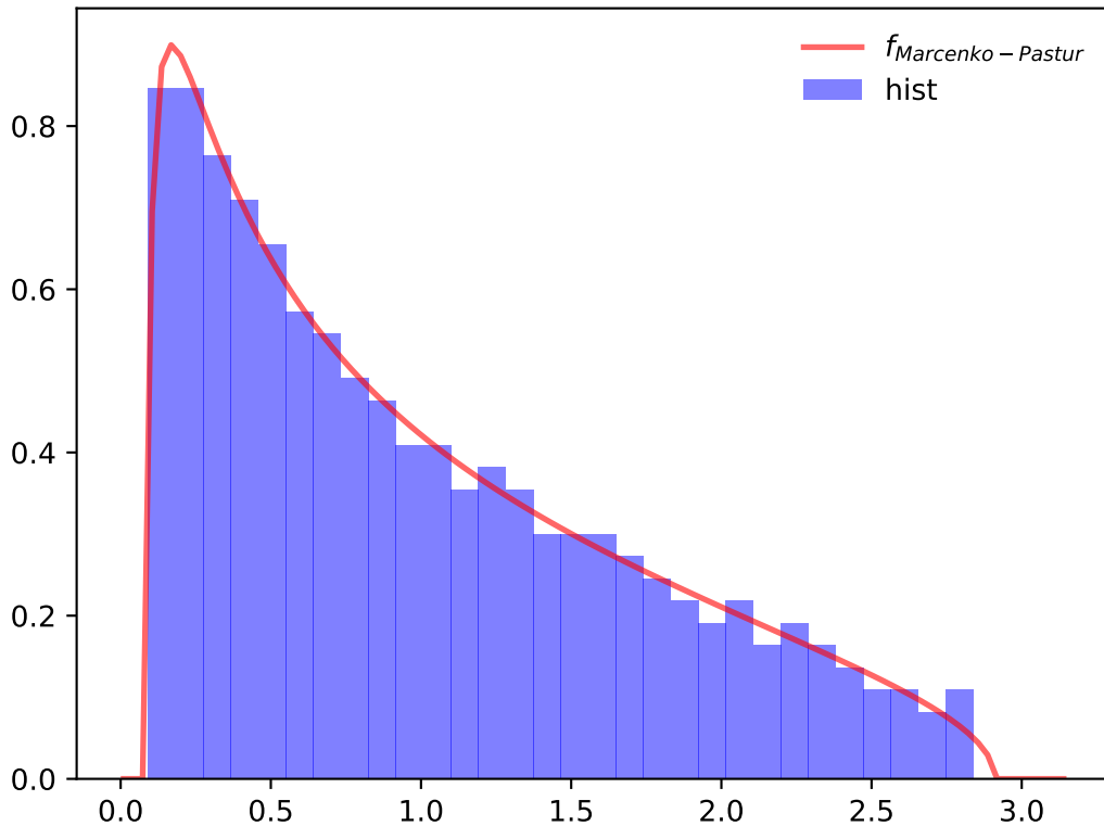
Realization of 400 points of Laguerre Ensemble with \beta = 2.98 with ratio M/N \approx 2.004
