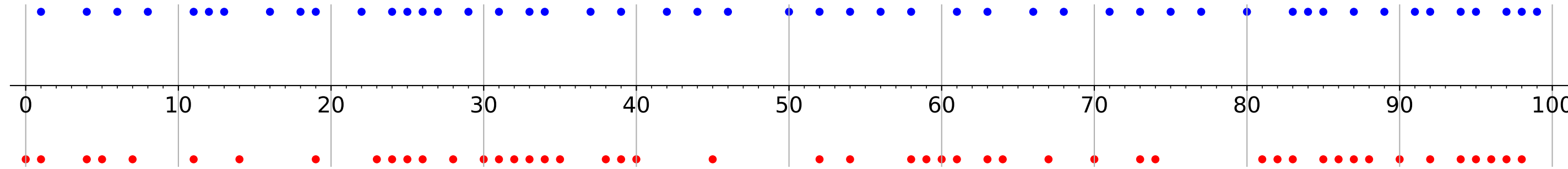
Realization of the Descent Process process vs independent Bernoulli variables with parameter p=0.500
