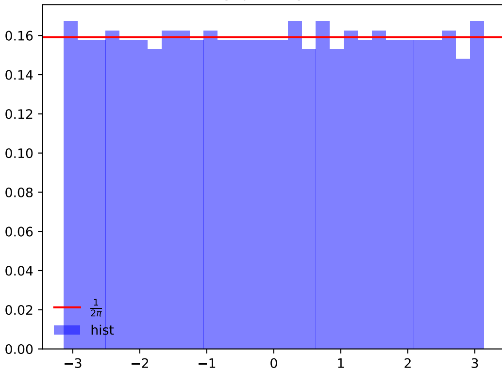
Realization of 1000 points of Circular Ensemble with \beta = 2 using quindiang model
