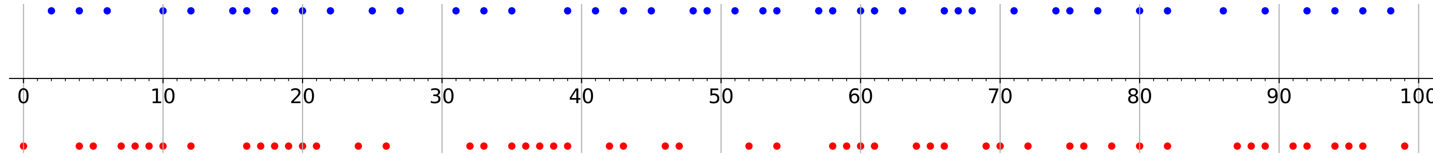
Realization of the Carries Process process vs independent Bernoulli variables with parameter p=0.450
