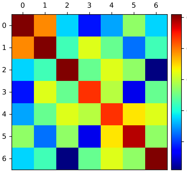
Correlation K kernel: transfer current matrix
