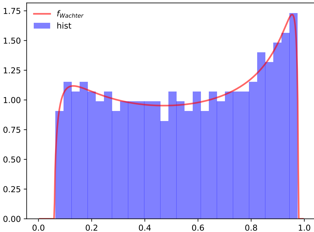
Realization of 400 points of Jacobi Ensemble with \beta = 3.14 with ratios, M_1/N \approx 1.794 , M_2/N \approx 1.475
