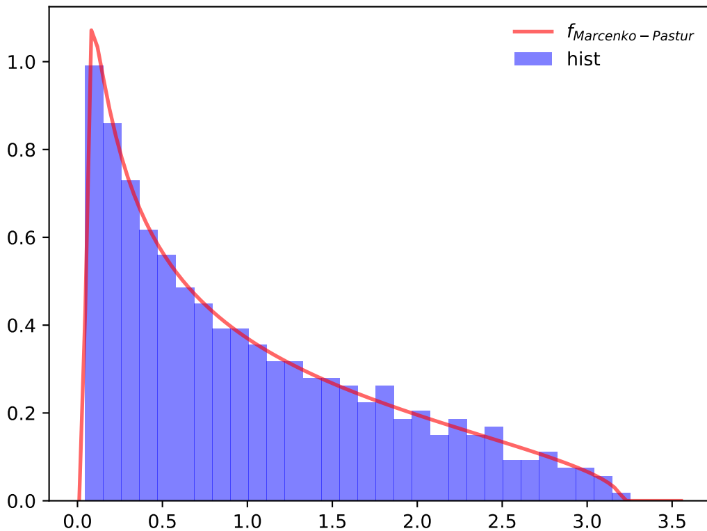
Realization of 500 points of Laguerre Ensemble with \beta = 1 with ratio M/N \approx 1.600
