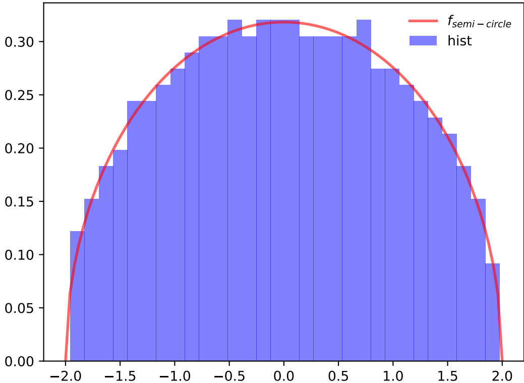
Realization of 500 points of Hermite Ensemble with \beta = 5.43
