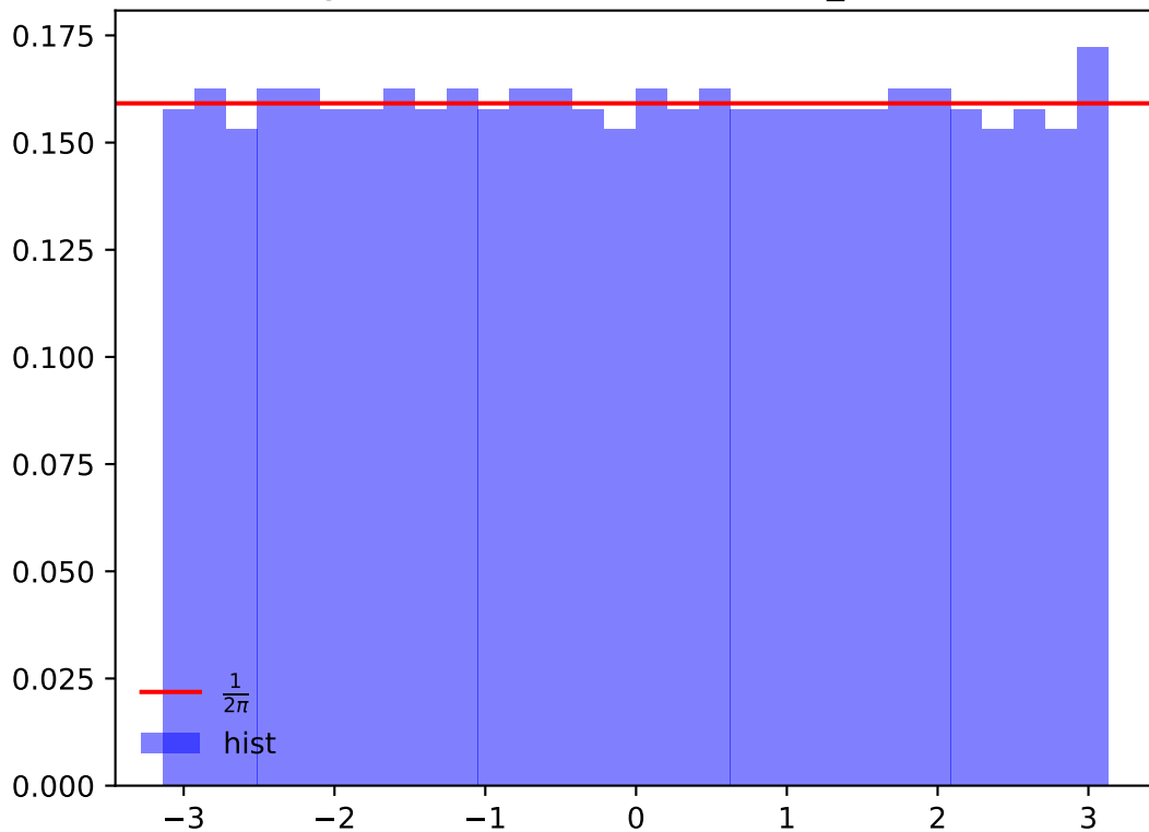
Realization of 1000 points of Circular Ensemble with \beta = 2 using full matrix model with haar_mode=QR
