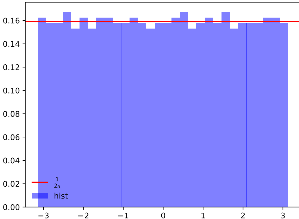
Realization of 1000 points of Circular Ensemble with \beta = 2 using full matrix model with haar_mode=Hermite
