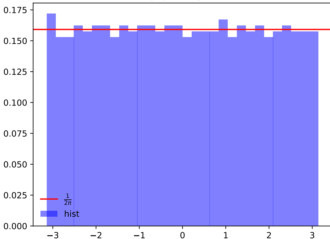
Realization of 1000 points of Circular Ensemble with \beta = 2 using quinddiag model
