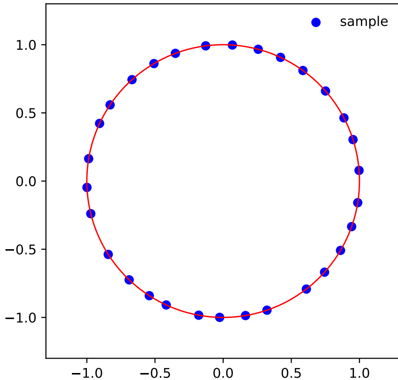
Realization of 30 points of Circular Ensemble with \beta = 10 using quindia model
